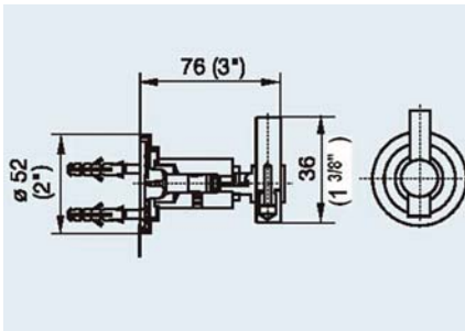
167/87 Temple Toilet Roll Holder
