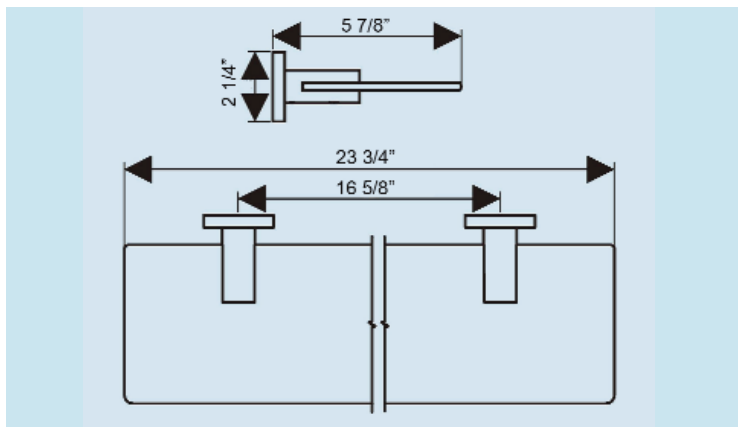
160/59 Nerea Glass Shelf
